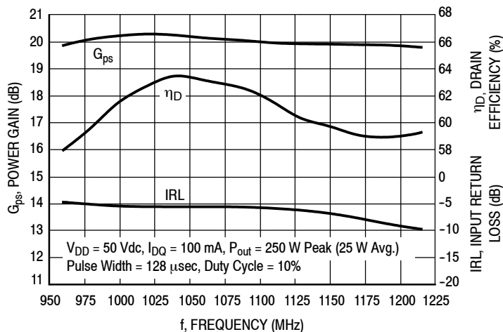
Figure 16. Broadband Performance @ P_{out} = 250 \text{ Watts Peak}
