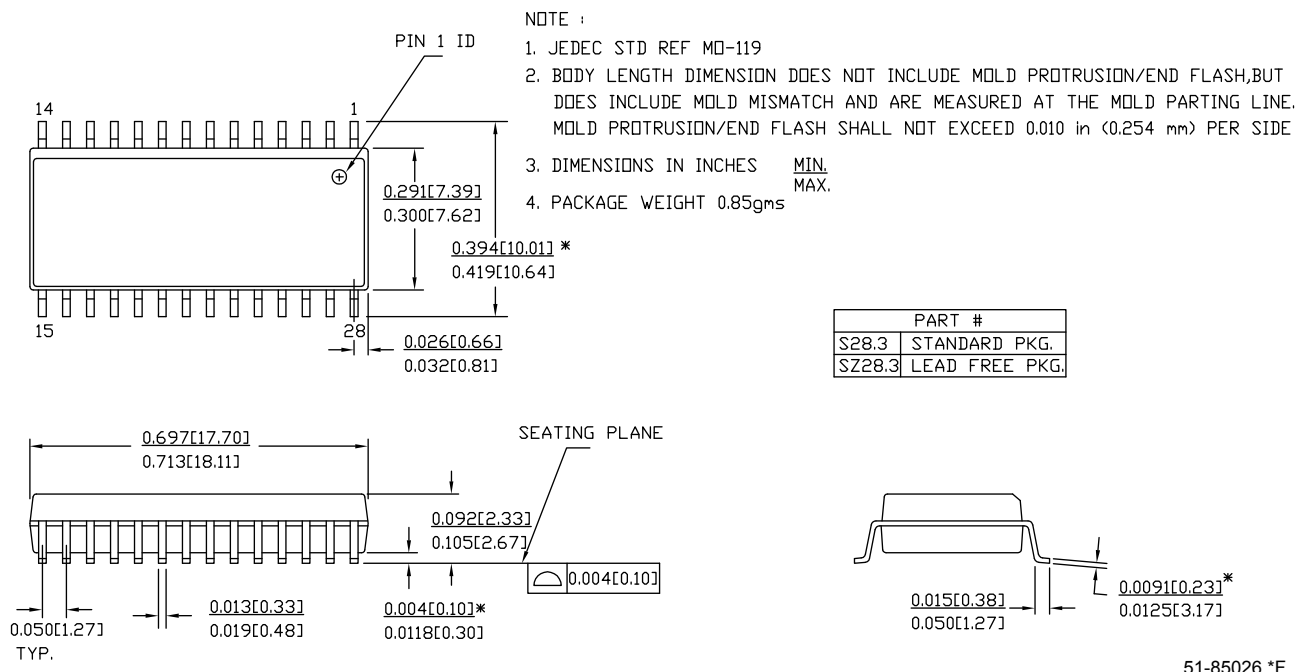
Figure 24. 28-pin (300-Mil) Molded SOIC
