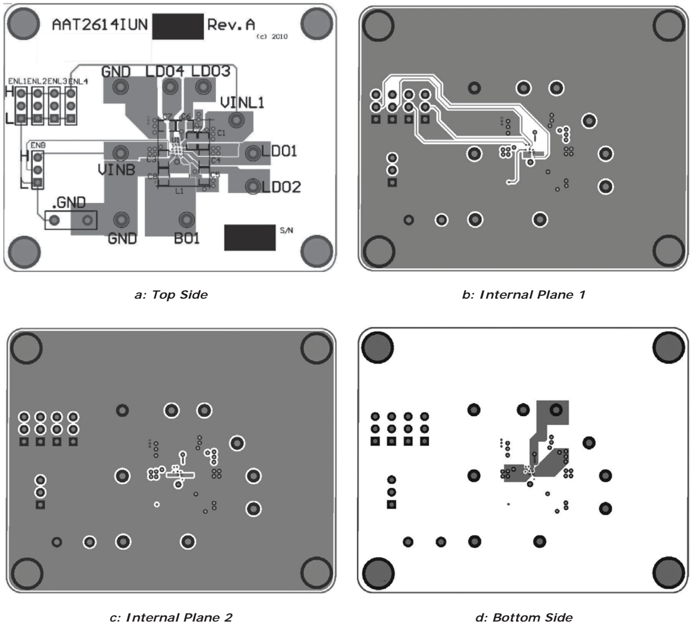
Figure 4: AAT2614IUN-2 Evaluation Board Layout.
