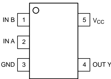
Figure 1. SC-88A (Top View)
