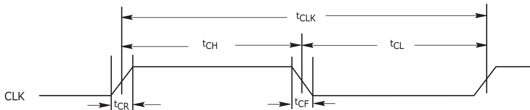
Figure 11.6 CLK Characterization
