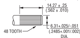
SHAFT TYPE "W" (USES BUSHING A)
