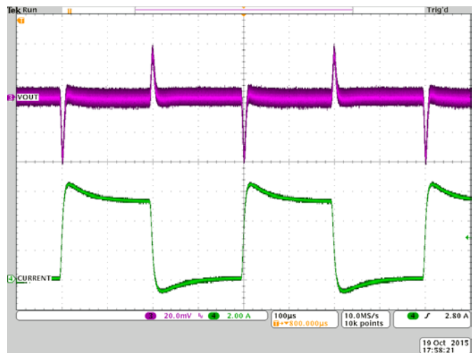
Figure 18: 0/6A load transient
