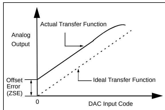
FIGURE 7-1: Offset Error Example.
