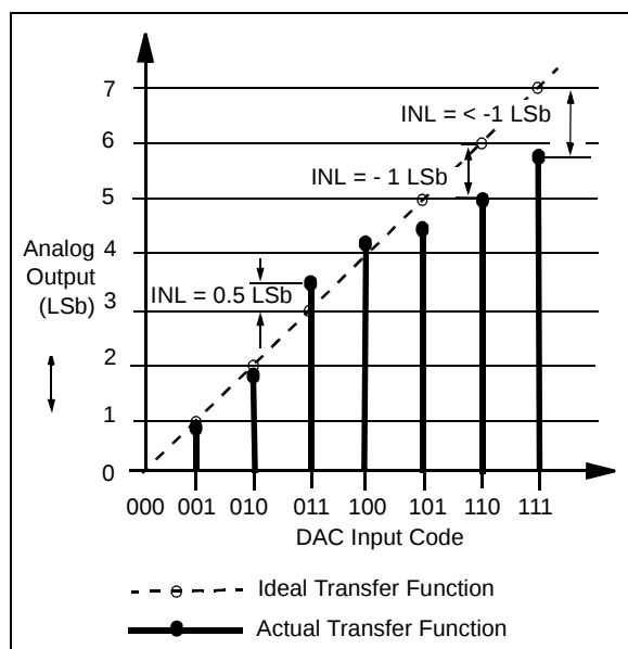
FIGURE 7-2: INL Accuracy Example.
