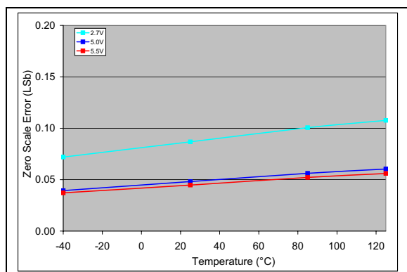
FIGURE 2-33: Zero-Scale Error (ZSE) vs. Temperature (MCP4706).
