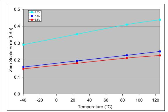
FIGURE 2-50: Zero-Scale Error (ZSE) vs. Temperature (MCP4716). V_{DD} = 5\text{V} , V_{REF1}:V_{REF0} = 11 , G = 0 , V_{REF} = V_{DD} .
