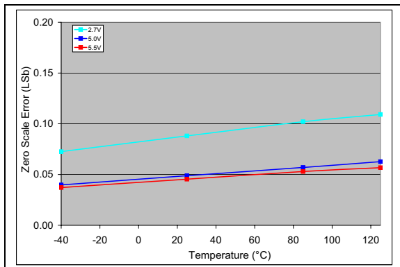
FIGURE 2-51: Zero-Scale Error (ZSE) vs. Temperature (MCP4706). V_{DD} = 5\text{V} , V_{REF1}:V_{REF0} = 11 , G = 0 , V_{REF} = V_{DD} .
