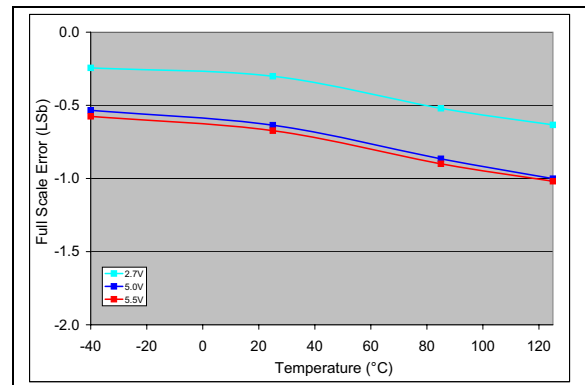
FIGURE 2-54: Full-Scale Error (FSE) vs. Temperature (MCP4706). V_{DD} = 2.7\text{V} , V_{REF1}:V_{REF0} = 11 , G = 0 , V_{REF} = V_{DD} .
