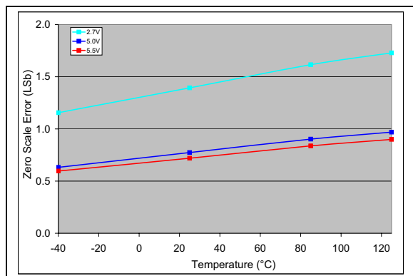
FIGURE 2-31: Zero-Scale Error (ZSE) vs. Temperature (MCP4726).
