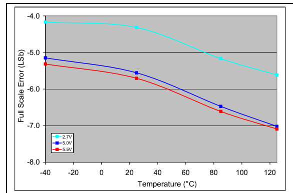
FIGURE 2-53: Full-Scale Error (FSE) vs. Temperature (MCP4716). V_{DD} = 2.7\text{V} , V_{REF1}:V_{REF0} = 11 , G = 0 , V_{REF} = V_{DD} .
