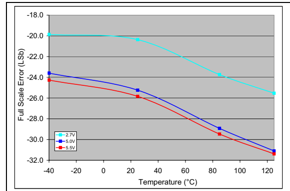
FIGURE 2-52: Full-Scale Error (FSE) vs. Temperature (MCP4726). V_{DD} = 2.7\text{V} , V_{REF1}:V_{REF0} = 11 , G = 0 , V_{REF} = V_{DD} .
