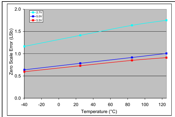
FIGURE 2-49: Zero-Scale Error (ZSE) vs. Temperature (MCP4726). V_{DD} = 5\text{V} , V_{REF1}:V_{REF0} = 11 , G = 0 , V_{REF} = V_{DD} .
