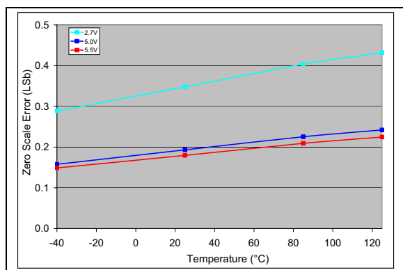
FIGURE 2-32: Zero-Scale Error (ZSE) vs. Temperature (MCP4716).
