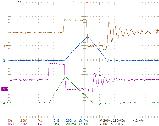
FIGURE 10. INDUCTOR CURRENT RIPPLE ( V_{IN} = 3.6V , PFM, INDUCTOR CURRENT RIPPLE = 200ns) CH1: SW1 (2V/DIV), CH2: IL1 (200mA/DIV), CH3: SW2 (2V/DIV), CH4: IL2 (200mA/DIV)
