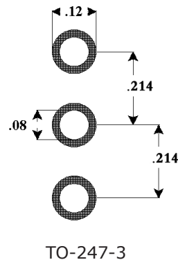
TO-247-3
