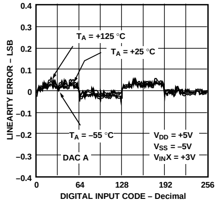
Figure 5. Linearity Error vs. Digital Code vs. Temperature
