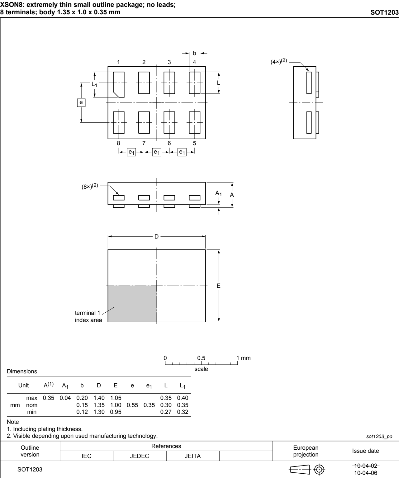
Figure 26. Package outline SOT1203 (XSON8)
