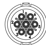
7 POSITION B-KEY #26 PIN & SOCKET CONTACT
