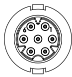
7 POSITION B-KEY #26 PIN & SOCKET CONTACT
