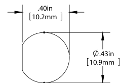
RECOMMENDED PANEL CUT-OUT TOLERANCE: \pm .003
