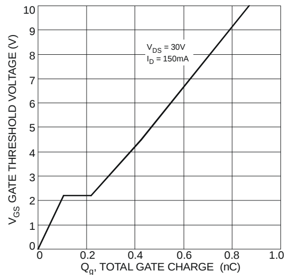
Figure 10 Gate Charge
