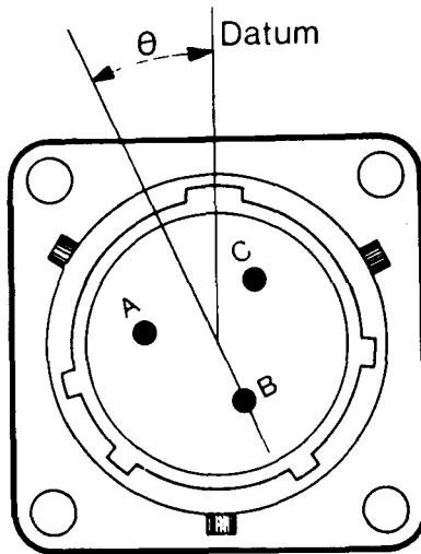
Alternative position of insert with socket contacts (Ø counter clockwise)
