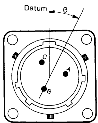
Alternate position of insert with pin contacts (Ø clockwise)
