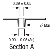
Figure 7. SC-79 Tape and Reel Dimensions
