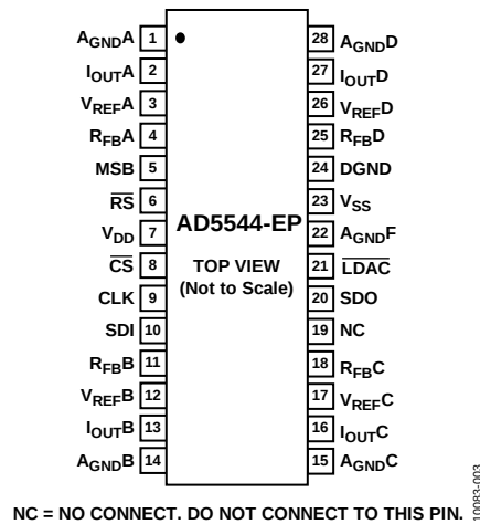
Figure 3. Pin Configuration
