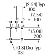
Momentary & Alternate
