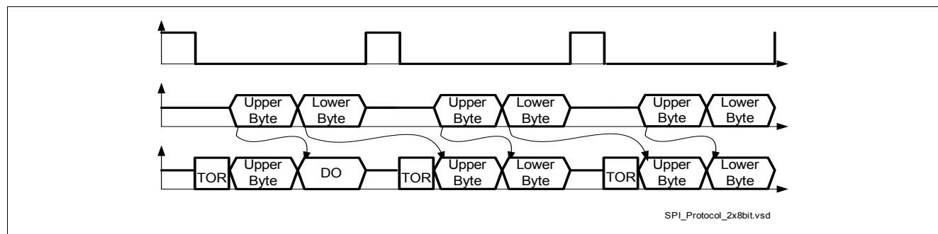
Figure 27 2x8-bit protocol
