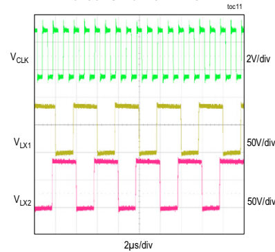
CLOCK SYNCHRONIZATION
