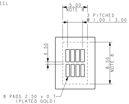
MATING PCB LAYOUT
