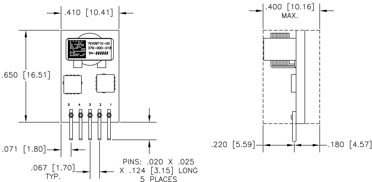
Figure 22. Mechanical Drawing
