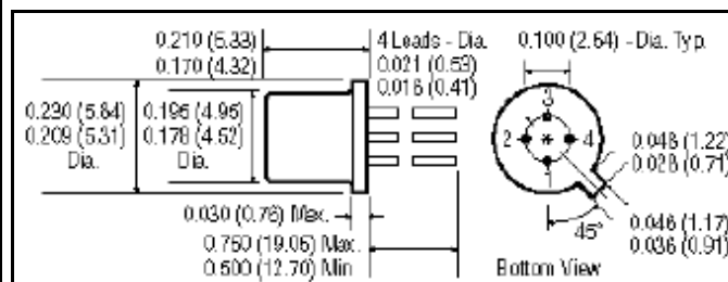
TO-72: 2N5397, 2N5398 1-Source, 2-Drain, 3-Gate, 4- Case
