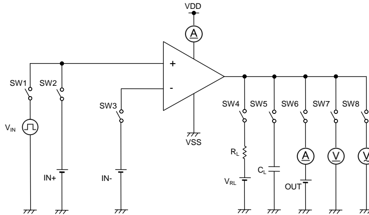
Figure 42. Test Circuit 2
