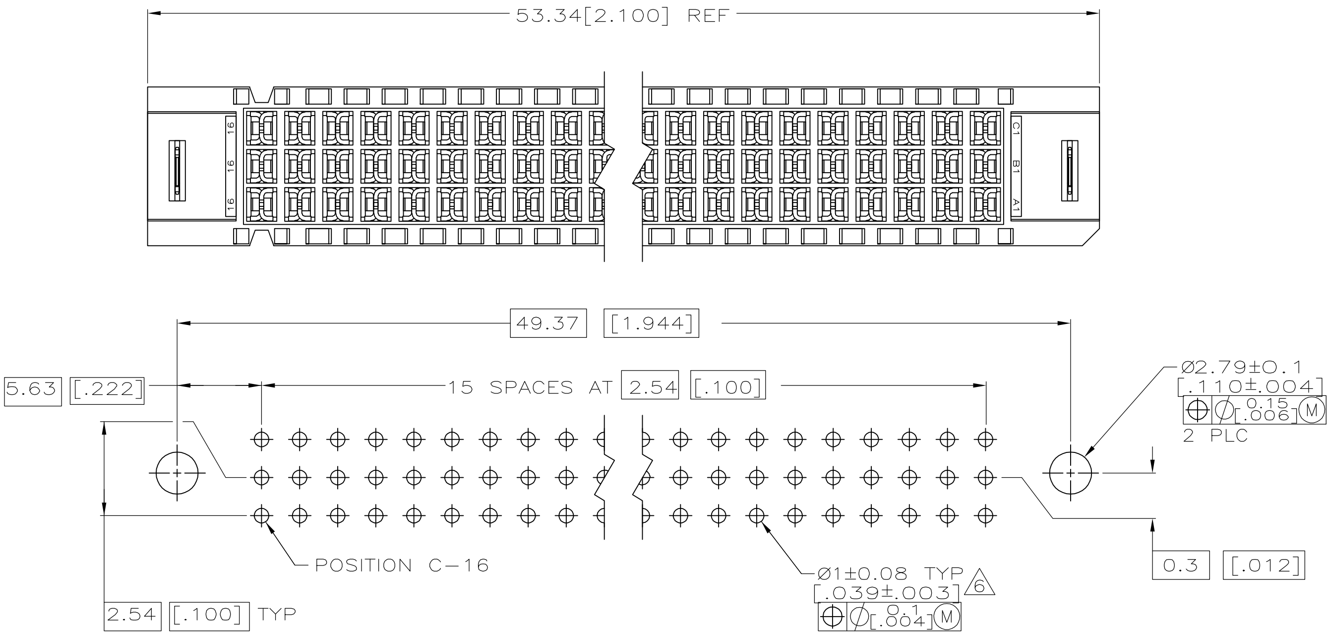
PC BOARD LAYOUT
