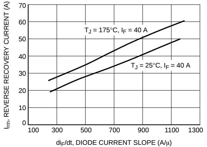
Figure 22. I_{rm} vs. di_F/dt ( V_R = 400 \text{ V} )
