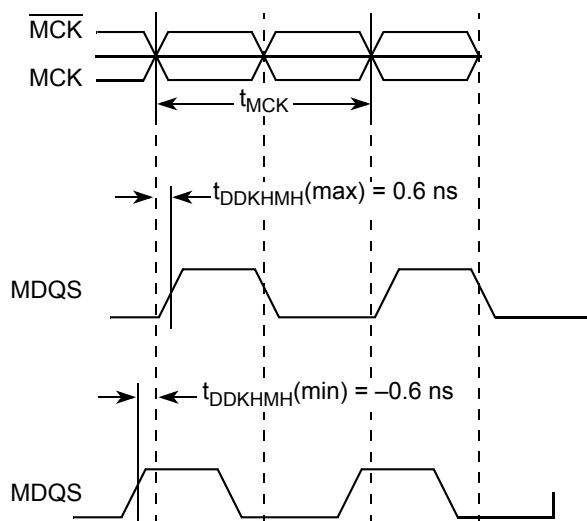
Figure 5. Timing Diagram for t_{DDKMH}
