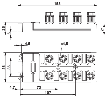
Dimensioned drawing
