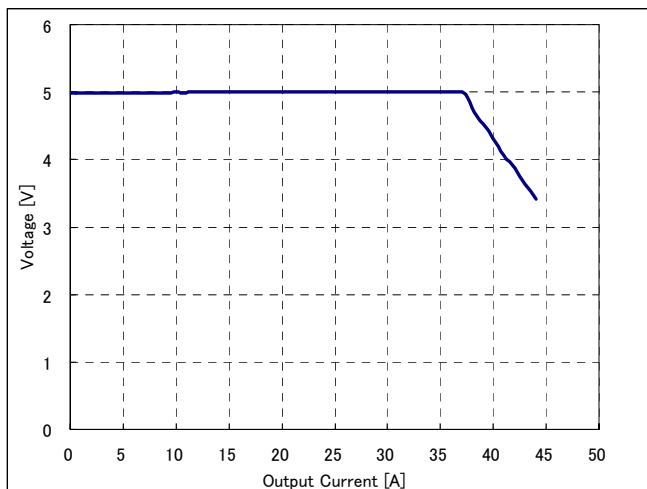
Fig-11: Output voltage vs. load current showing current limit point and converter shutdown point. ( V_{in} = 48\text{V} )
