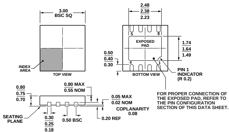
Figure 58. 8-Lead Lead Frame Chip Scale Package [LFCSWP_WD] 3 mm × 3 mm Body, Very Very Thin, Dual Lead (CP-8-5)
