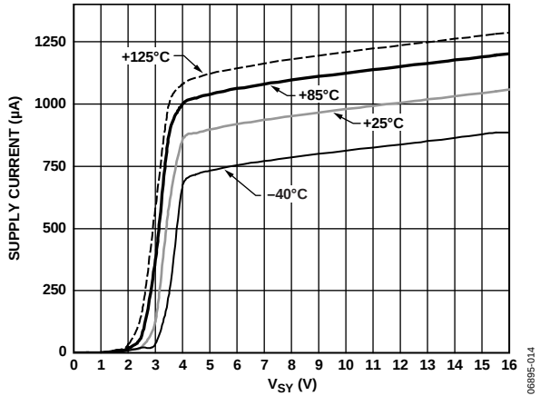
Figure 43. Supply Current vs. Supply Voltage
