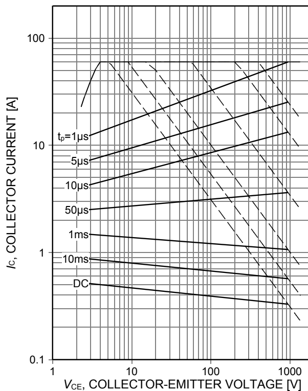
Figure 2. Forward bias safe operating area (D=0, T_C=25^\circ\text{C}, T_{vj} \leq 175^\circ\text{C}; V_{GE}=15\text{V})
