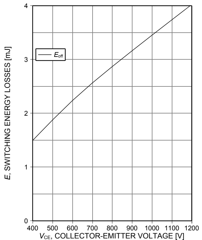
Figure 16. Typical switching energy losses as a function of collector emitter voltage (inductive load, T_{vj}=175^\circ\text{C} , V_{GE}=0/15\text{V} , I_C=20\text{A} , R_{G(on)}=15\Omega , R_{G(off)}=15\Omega , dynamic test circuit in Figure E)
