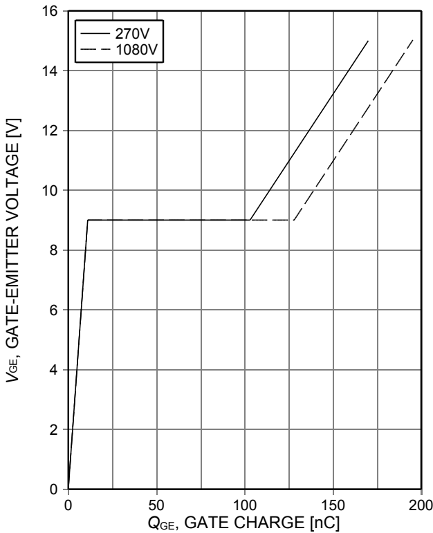
Figure 18. Typical gate charge ( I_C=20\text{A} )
