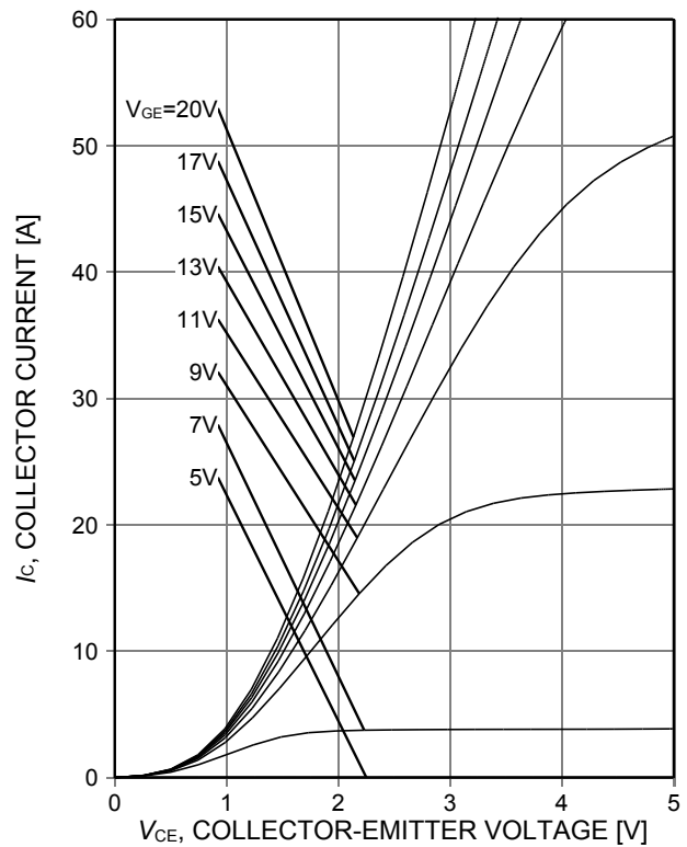
Figure 6. Typical output characteristic ( T_{vj}=175^{\circ}\text{C} )
