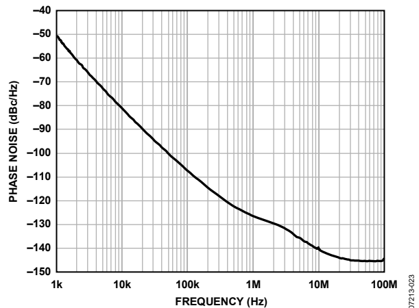
Figure 23. Internal VCO Phase Noise (Absolute), Direct-to-LVPECL @ 2550 MHz
