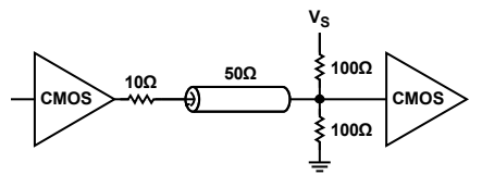
Figure 74. CMOS Output with Far-End Termination
