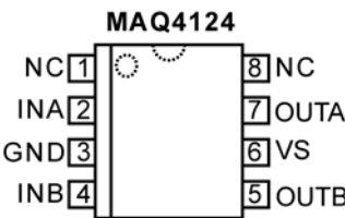
DUAL NON-INVERTING
