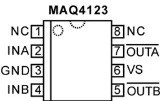
DUAL INVERTING
