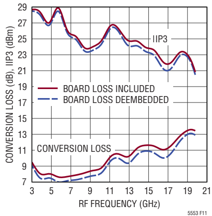
Figure 11. Comparison of the LTC5553 Performance Before and After De-Embedding the Insertion Loss of the Evaluation Board and SMA Connectors. Downconversion Application with Low Side LO, IF = 1890MHz, V_{CC} = 3.3V , EN = High, T_C = 25^\circ C
