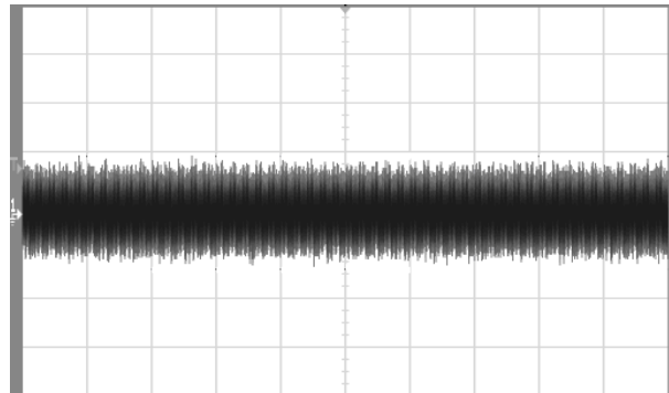
Figure 3 Input reflected ripple current (100ms/div, 10mA/div), see Figure 14 for test configuration
