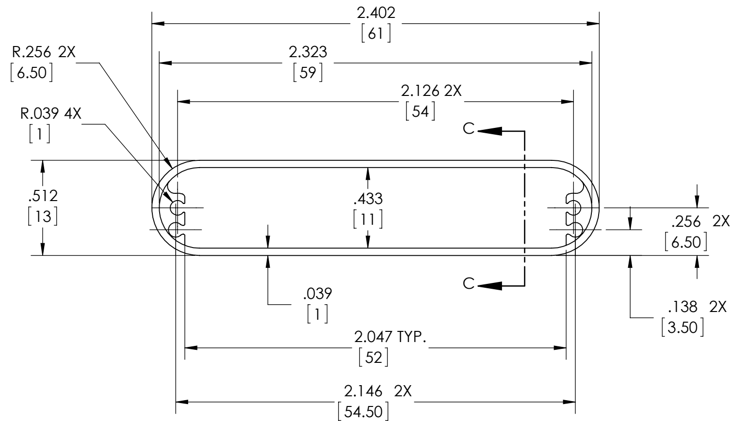
EXTRUSION PROFILE
