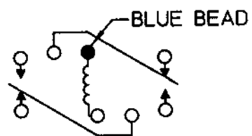
TERMINAL VIEW
