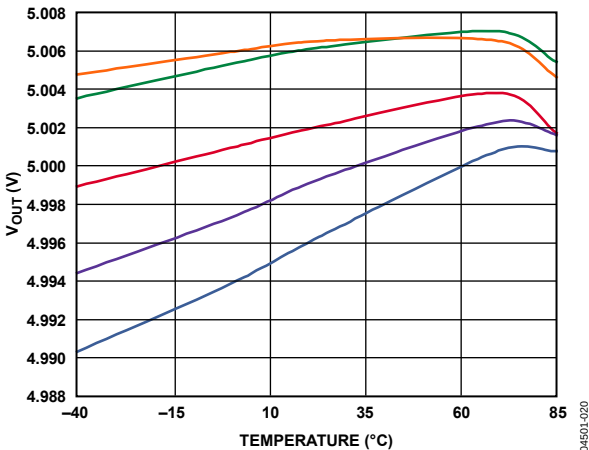
Figure 17. Data for Five Parts of ADR550 V_{OUT} over Temperature
