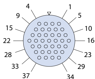
Size 3-37 37 Contacts
