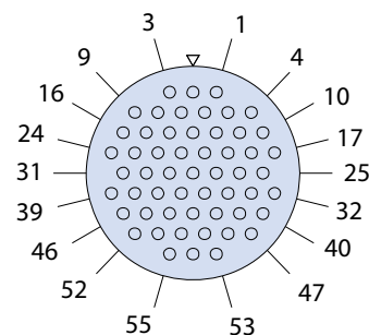
Size 4-55 55 Contacts
