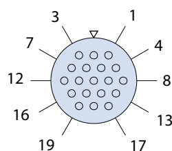
Size 2-19 19 Contacts
