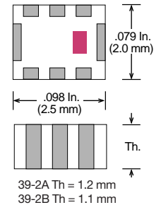
Case 39-2 (2520)
