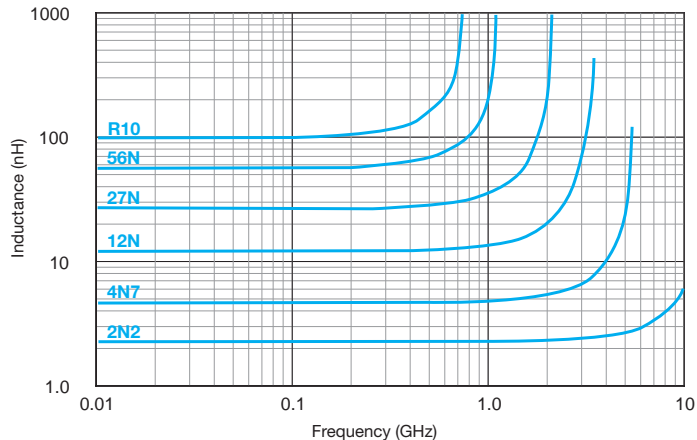
INDUCTANCE VS FREQUENCY: SIZE 0603
