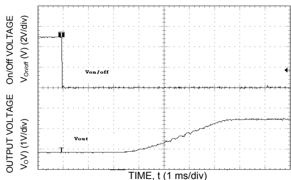
Figure 15. Typical Start-Up Using Remote On/Off with Low-ESR external capacitors (7x150 \mu F Polymer) ( V_{in} = 12 Vdc, V_o = 3.3 Vdc, I_o = 5.0 A, C_o = 1050\mu F).
