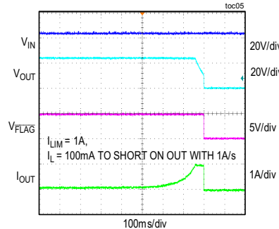
CURRENT-LIMIT RESPONSE
