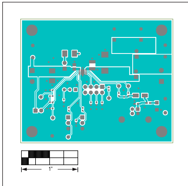
MAX17608 EV Kit PCB Layout—Top Layer
