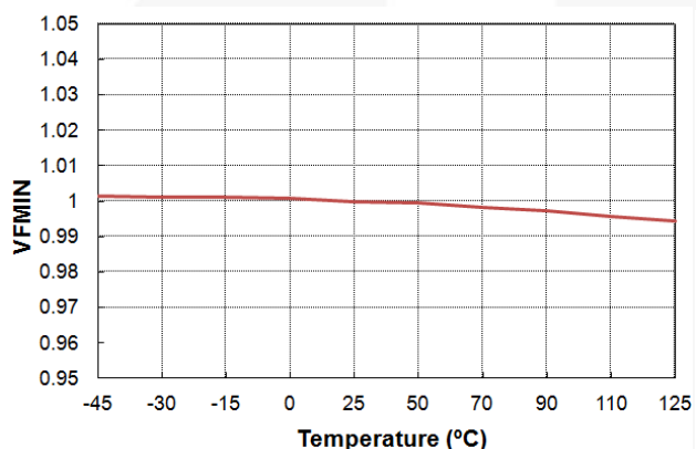
Figure 6. VFMIN vs. Temperature
