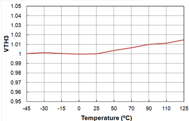
Figure 43. VTH3 vs. Temperature
