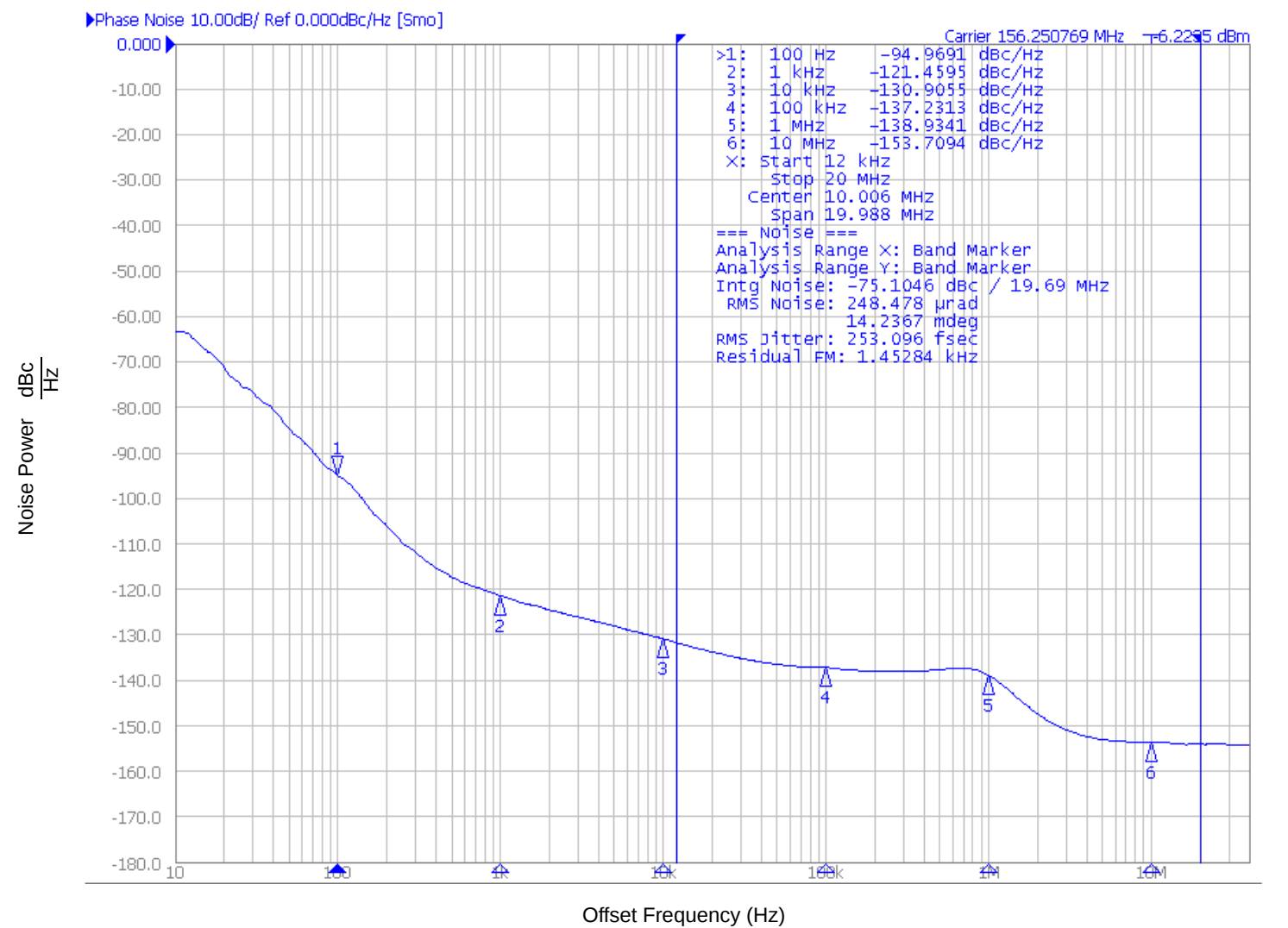
RMS Phase Noise (Random) for Integer PLL Feedback and f_{\text{XTAL}}=100.000\text{MHz} .
